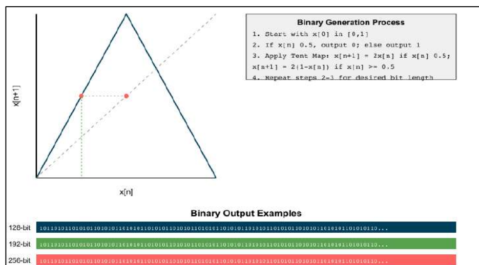
Figure 7: Tent Map for Generating Binary Numbers
