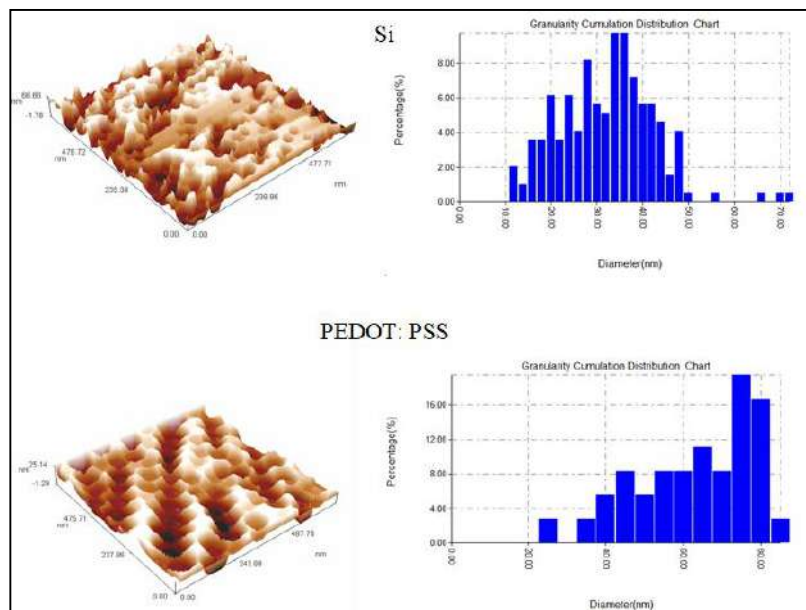
Figure 3: Displays a 3D image with a Chart depicting the dispersion of granular accumulations(a) Si and (b) PEDOT: PSS for AFM analysis.
