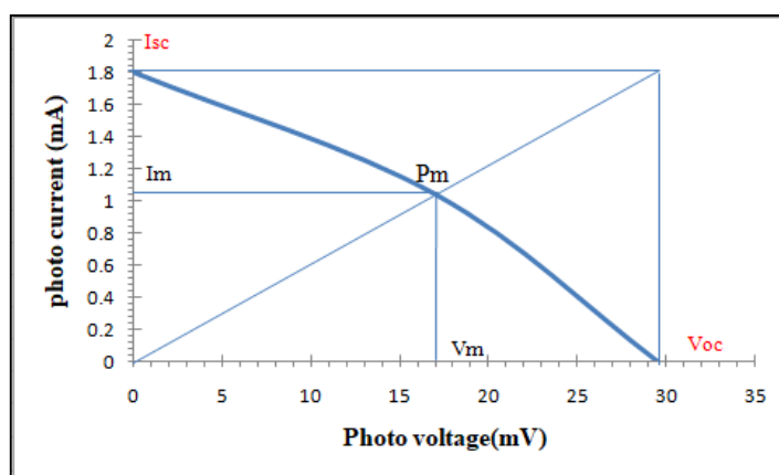
Figure 7: PEDOT: PSS solar cell I-V curve
